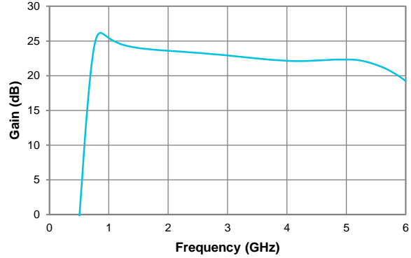
Insertion Gain
